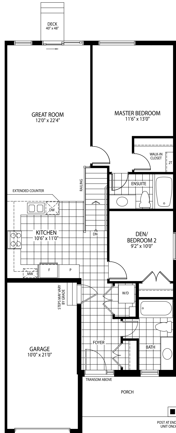
GROUND FLOOR PLAN END UNIT
