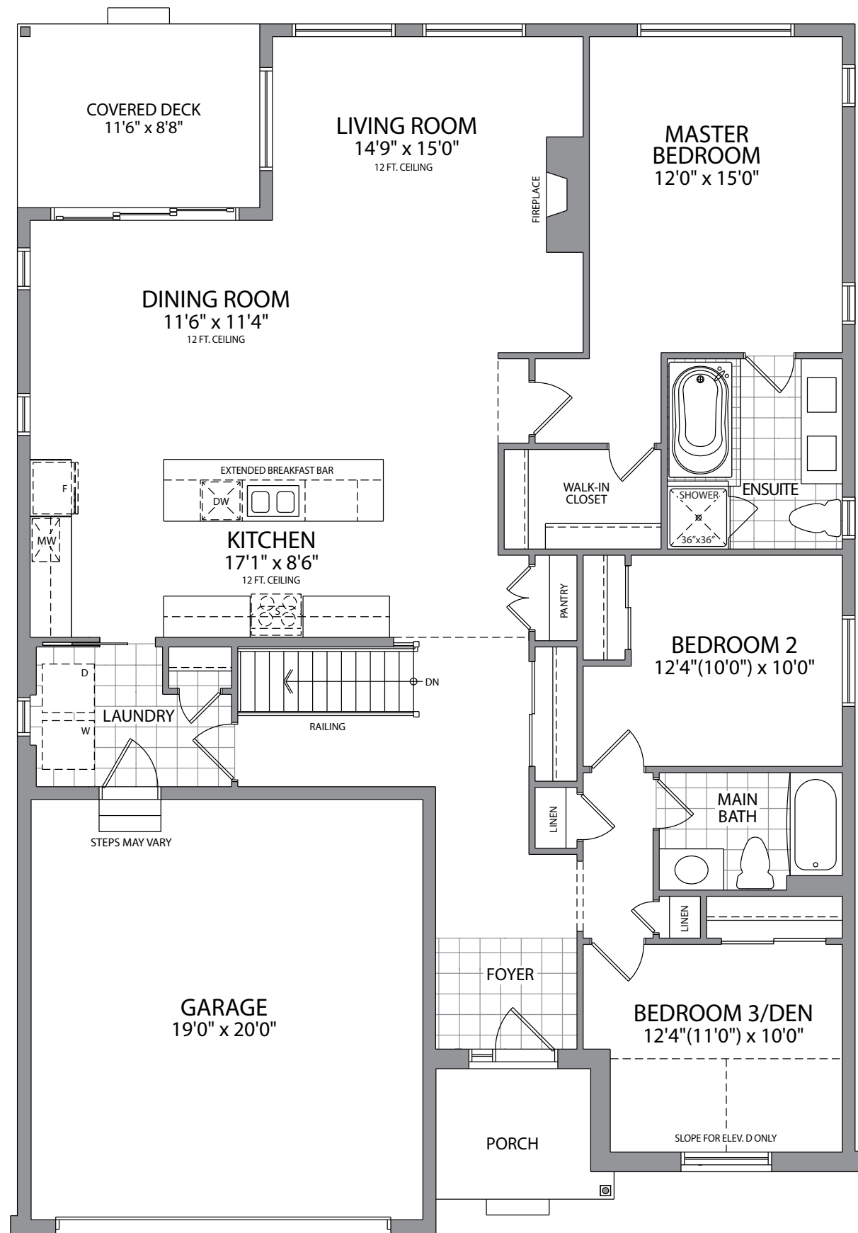
GROUND FLOOR* ELEV. B & D
