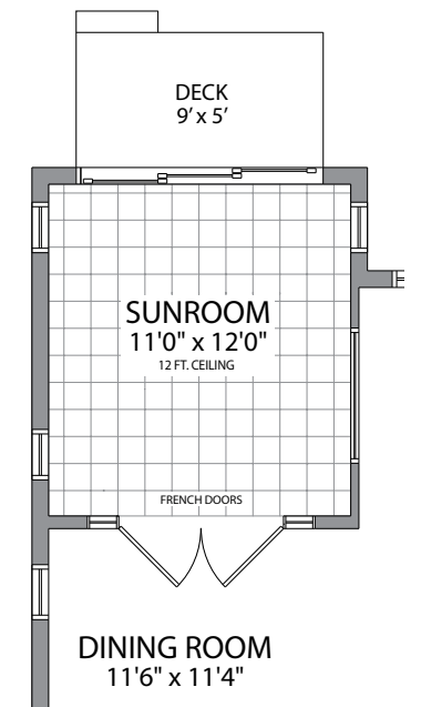
OPT. SUNROOM 148 SQ. FT.
