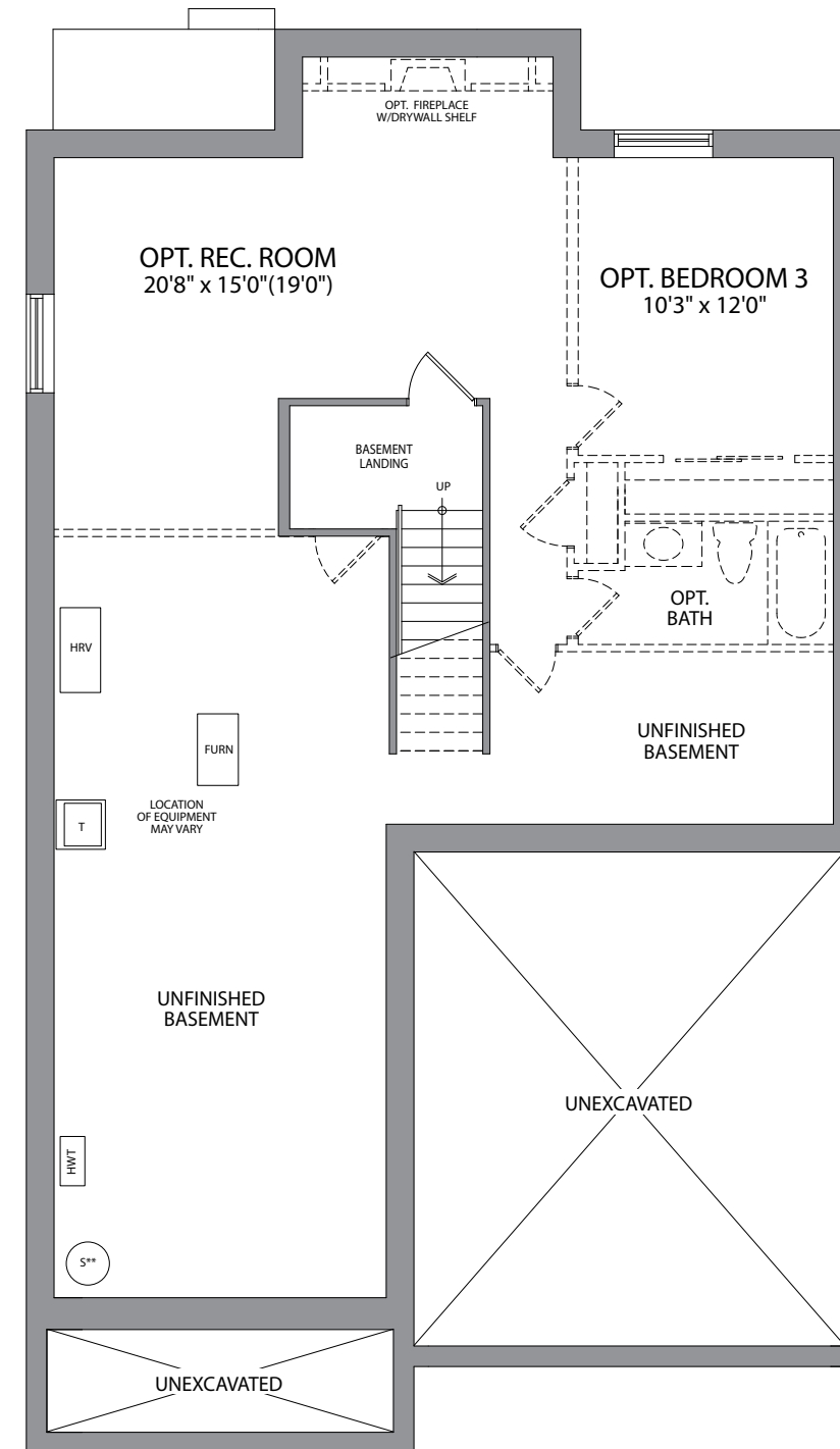
BASEMENT OPT. FINISHED BASEMENT 625 ft 2
